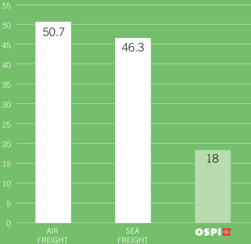
CO 2 EMISSIONS IN TONS
